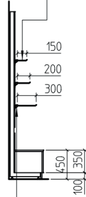
AX-Hanging Rail T15 X 30
