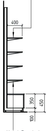
Metal Bracket for SDB Panel Shelf
